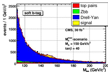
Fig. 3. Invariant di-muon distribution for the H/A \rightarrow \mu^+\mu^- signal with m_A = 150 \text{GeV}/c^2 and \tan\beta = 40 and for the total background for 30 \text{ fb}^{-1} in CMS.
