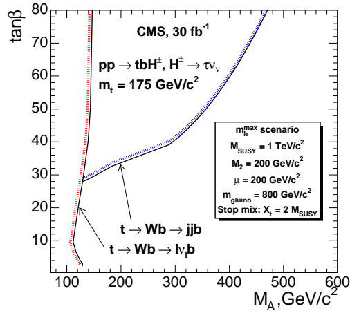
Fig. 6. Discovery potential of CMS for the charged MSSM Higgs bosons H^\pm with the H^\pm \rightarrow \tau\nu_\tau decay mode for 30 \text{ fb}^{-1} .
