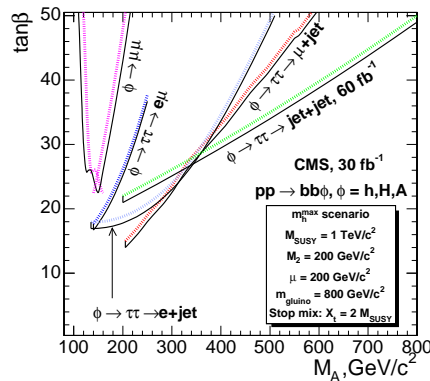
Fig. 2. Discovery potential of CMS for the heavy neutral MSSM Higgs bosons H and A with the H/A \rightarrow \mu^+\mu^- and H/A \rightarrow \tau^+\tau^- decay channels for 30 and 60 \text{fb}^{-1} .
