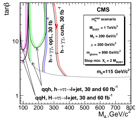
Fig. 1. Discovery potential of CMS for the lighter scalar MSSM Higgs boson h with the h \rightarrow \gamma\gamma and h \rightarrow \tau^+\tau^- \rightarrow \ell + \text{jet} channels for 30 and 60 fb ^{-1} .
