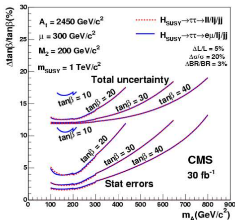
Fig. 4. Expected precision of \tan\beta measurement from the event rates in the H/A \rightarrow \tau^+\tau^- decay channels as a function of m_A and \tan\beta for 30 \text{ fb}^{-1} in the CMS detector.
