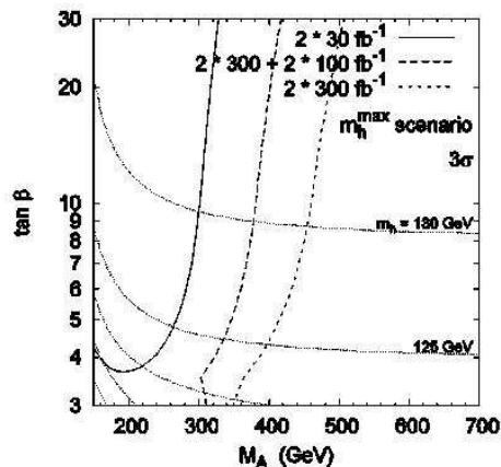
Fig. 5. Regions of the MSSM parameter space, where the discrepancy between SM and the MSSM is larger than 3\sigma for three different integrated luminosities in the ATLAS detector. The fits are based on the h measurements alone.
